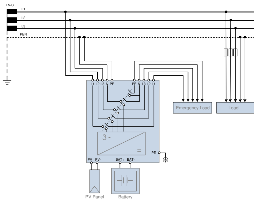
Fig-1 TN-C System
